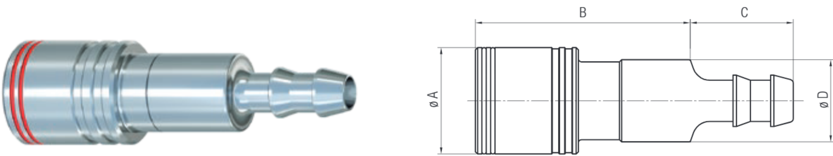
Push-on Female
