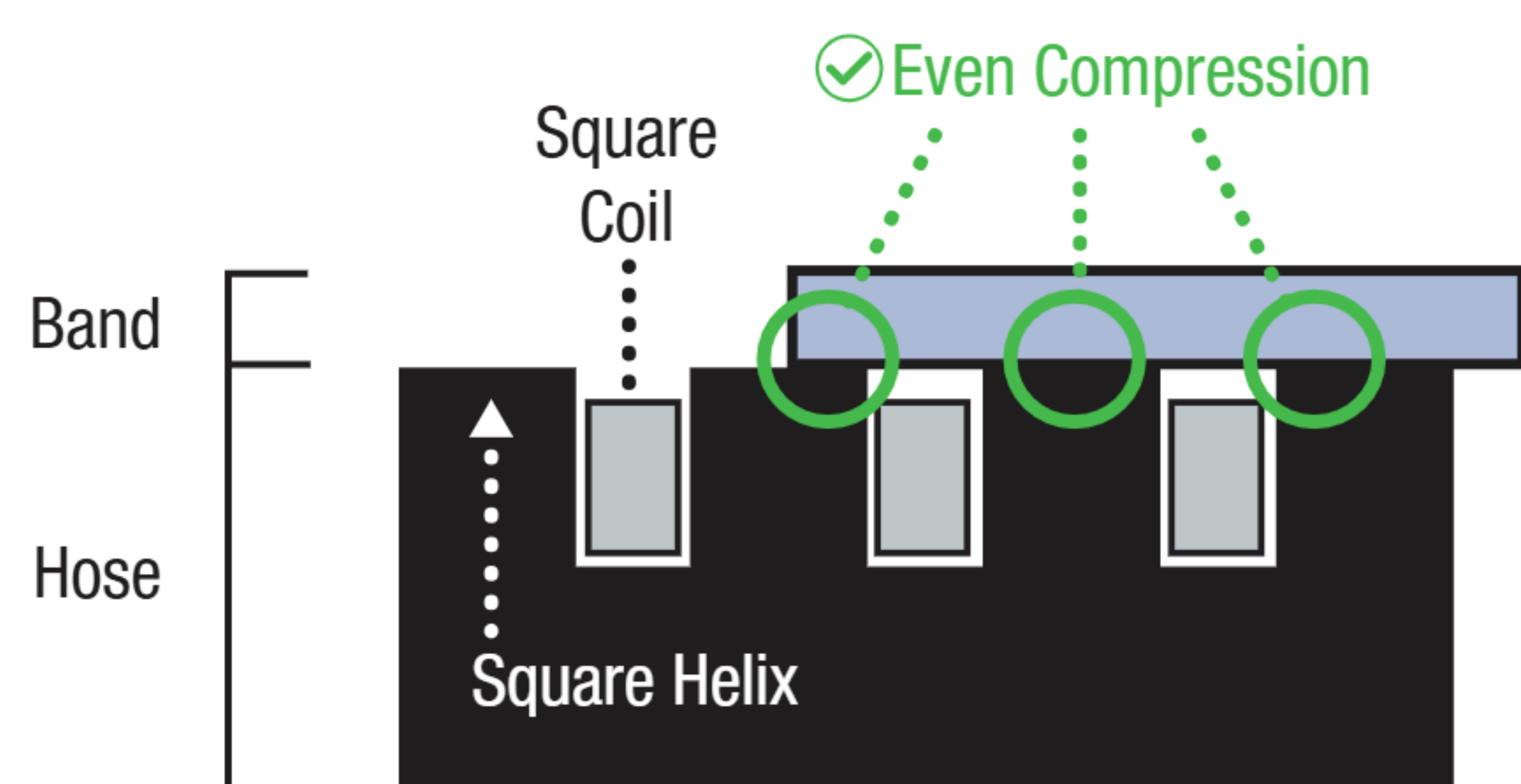
Square Design = Greater Compression
