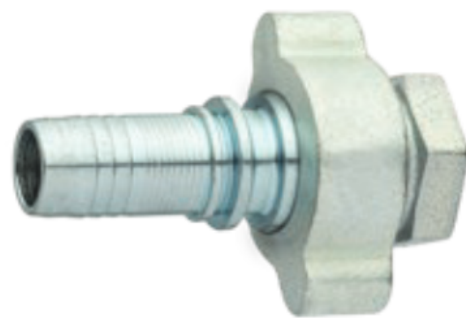
Female Crimp Ground Joint with Wing Nut and Female NPT Spud
