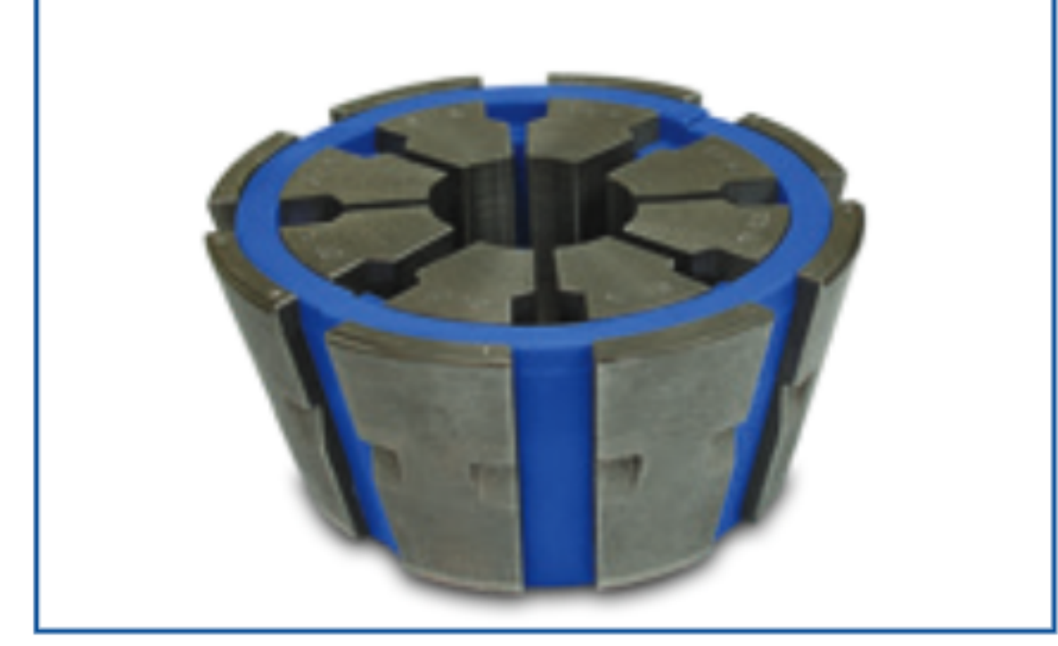
T400 22.2mm Die Set P/N: PF402-22.2D
